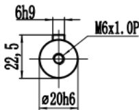
输出轴径/Output Diameter
