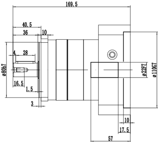
输出轴径/Output Diameter
